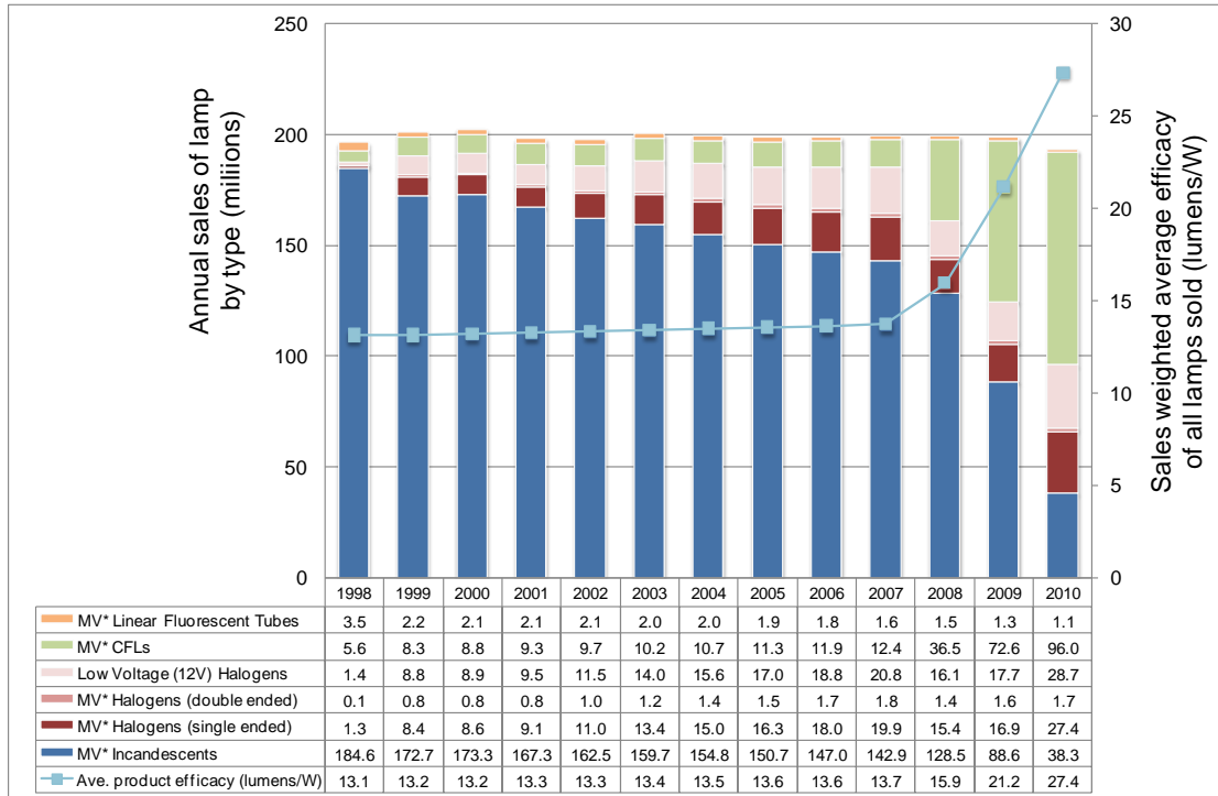
Figure 20. Time series lamp sales by type in the UK.
